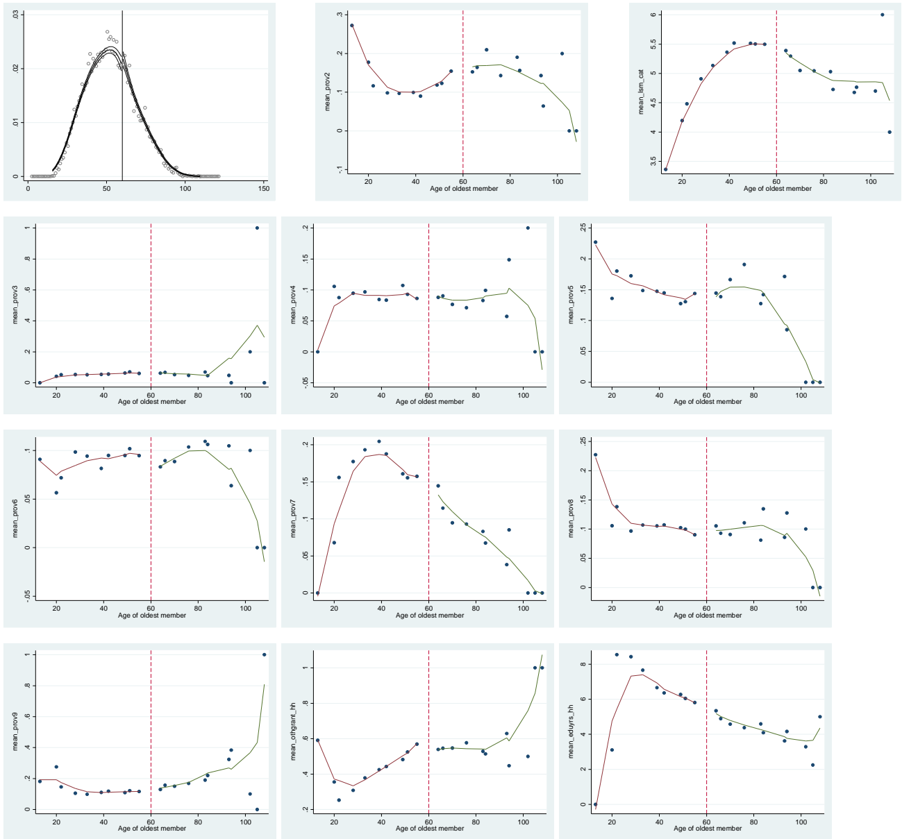
Figure 8: Checking for Balanced Covariates
