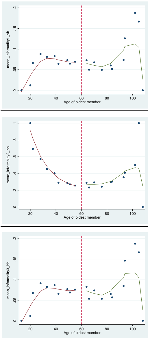
Figure 9: Checking for Discontinuities in the Outcome Variable
